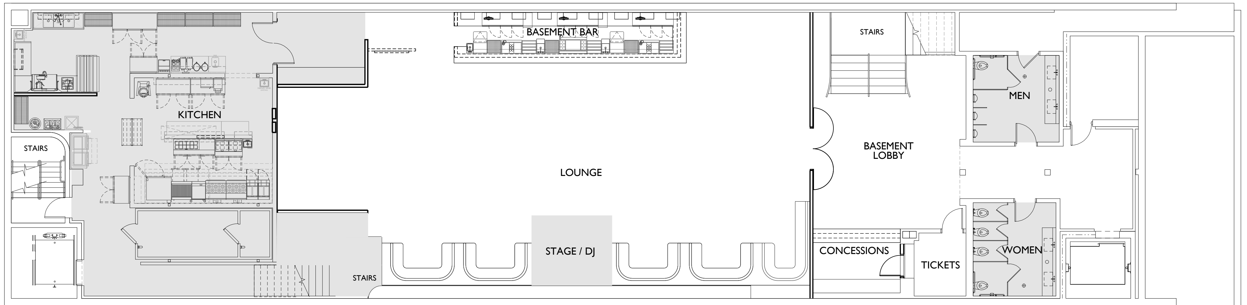
LOUNGE LEVEL FLOOR PLAN
